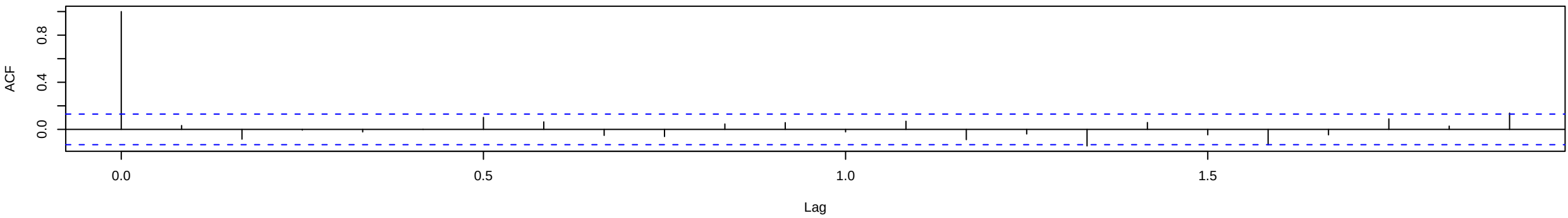
ACF of Residuals
