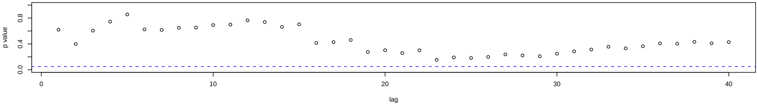
p values for Ljung-Box statistic
