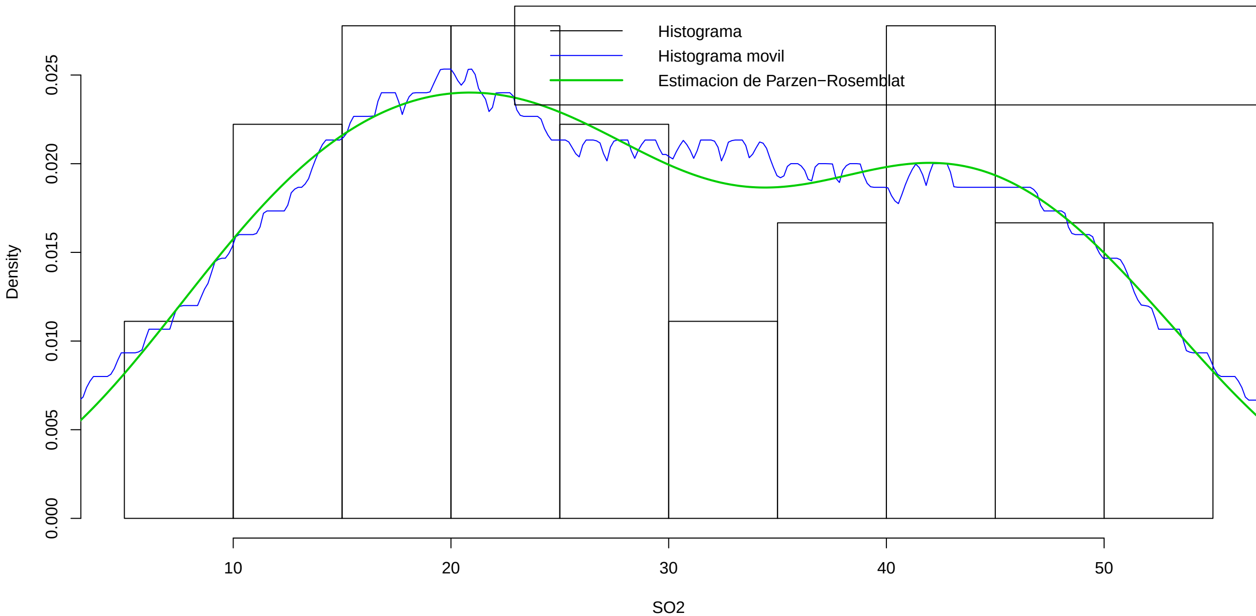
Histogram of SO2
