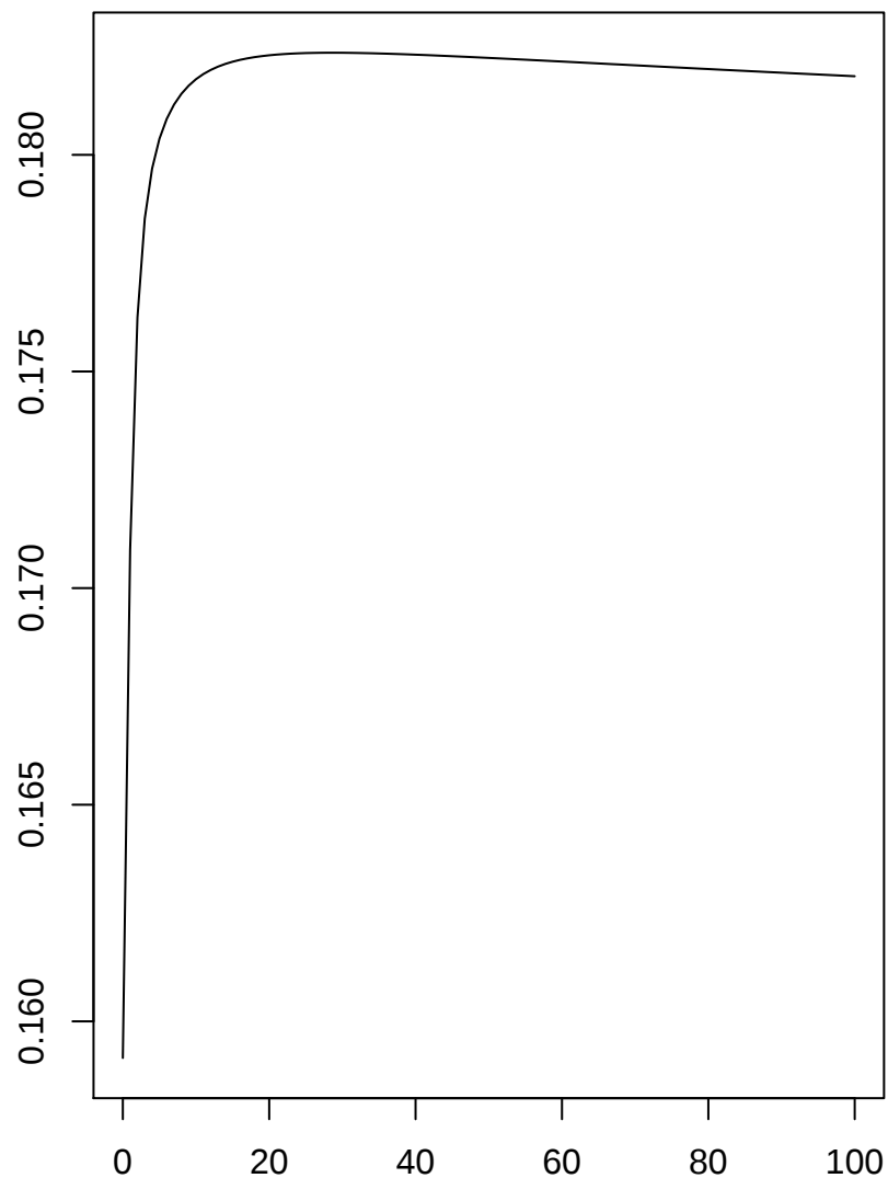
Cross validation. Squared-error loss
