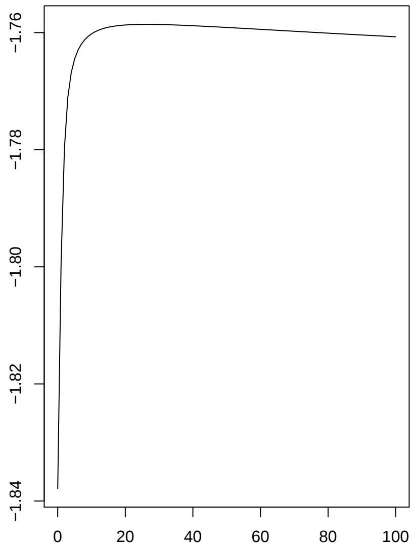
Cross validation. Kullback-Leibler
