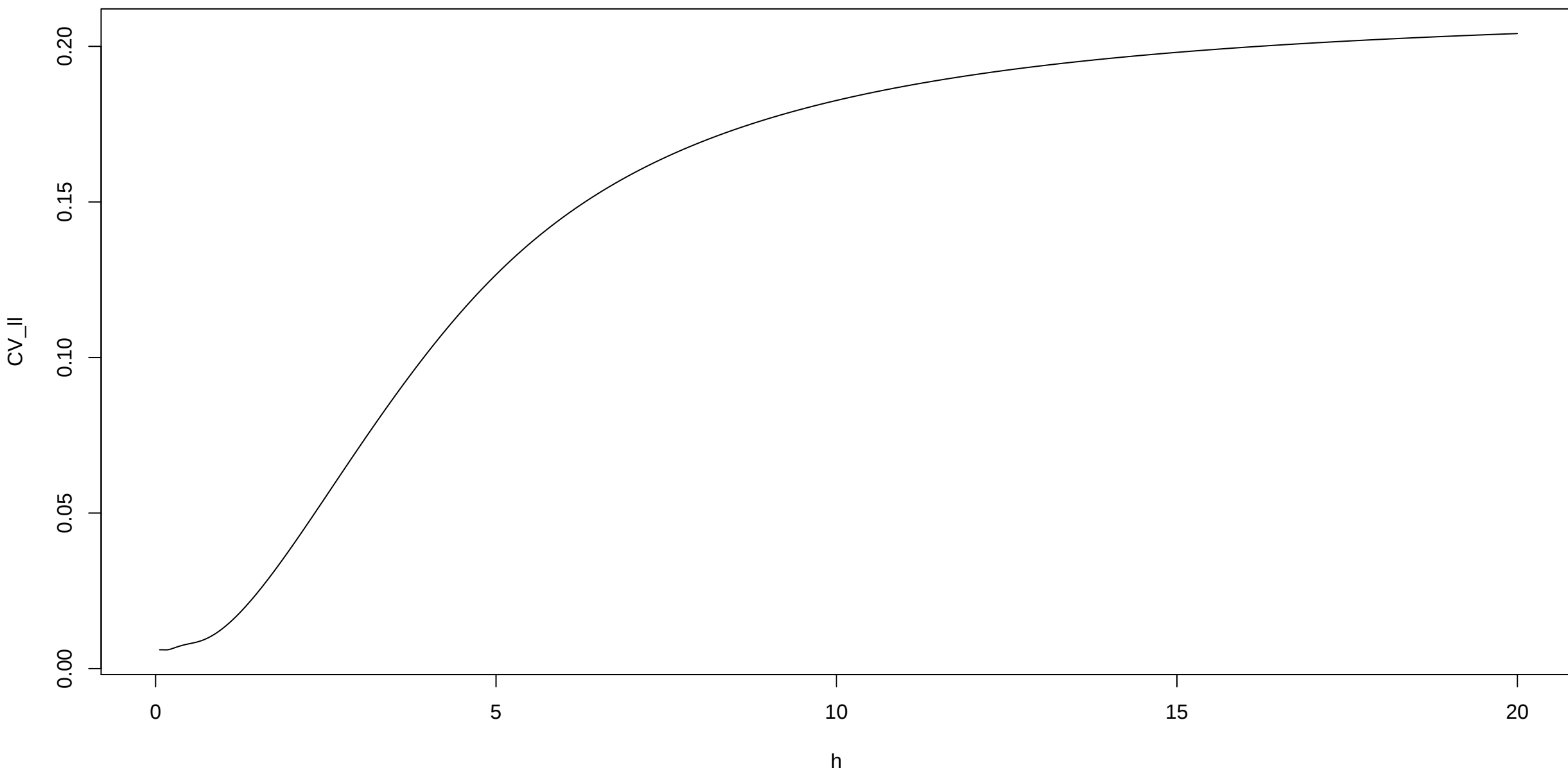
cross validation Linear-local
