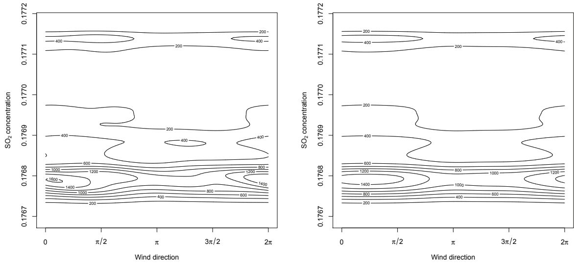
Figure 9: Monitoring station G2. Contour plot for joint density estimator for wind direction and \text{SO}_2 concentrations (left plot). Joint density estimation under independence (right plot).
