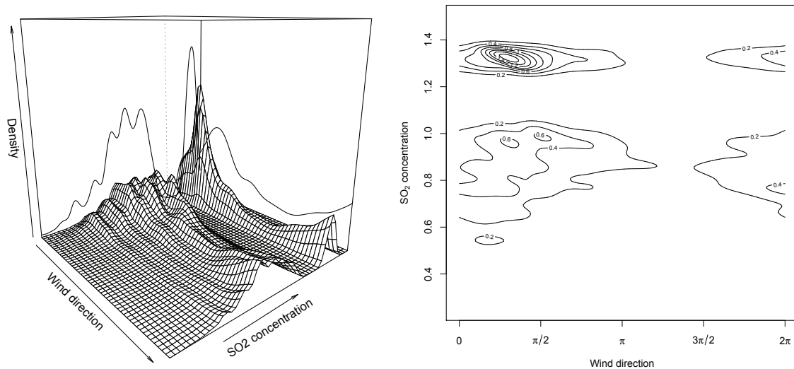
Figure 6: Monitoring station B1. Joint density estimator for wind direction and \text{SO}_2 concentrations.
