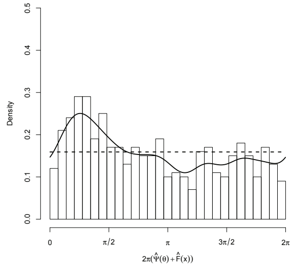
Figure 5: Monitoring station B1. Solid line: joining density estimator using circular kernel method with cross-validated bandwidth. Dashed line: circular uniform density. Histogram for artificial sample \{2\pi(\hat{\Psi}(\theta_i) + \hat{F}(x_i))\}_{i=1}^n .
