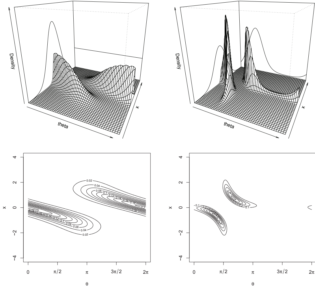
Figure 3: Left column: Example 1 density surface with parameters \mu = \pi and \kappa = 2 . Right column: Example 2 density surface with parameters \mu = \pi , \kappa = 5 , \mu_1 = \frac{\pi}{2} and \kappa_1 = 2 .
