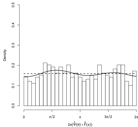
Figure 8: Monitoring station G2. Solid line: joining density estimator using circular kernel method with cross–validatory bandwidth. Dashed line: circular uniform density. Histogram for artificial sample \{2\pi(\hat{\Psi}(\theta_i) + \hat{F}(x_i))\}_{i=1}^n .
