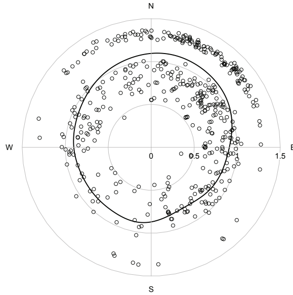
Figure 7: Monitoring station B1. Nadaraya–Watson estimator (solid line) with circular explanatory variable for \text{SO}_2 over wind direction, with cross–validatory bandwidth. \text{SO}_2 concentrations are shown in the horizontal axis.
