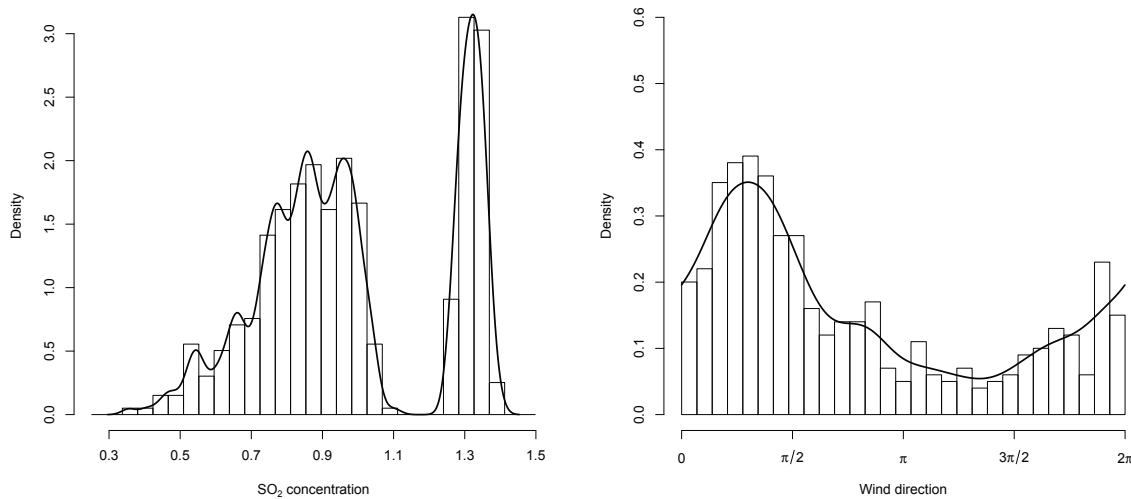
Figure 4: Monitoring station B1. Marginal densities estimators for \text{SO}_2 and wind direction, using linear and circular kernel density with cross-validated bandwidths.
