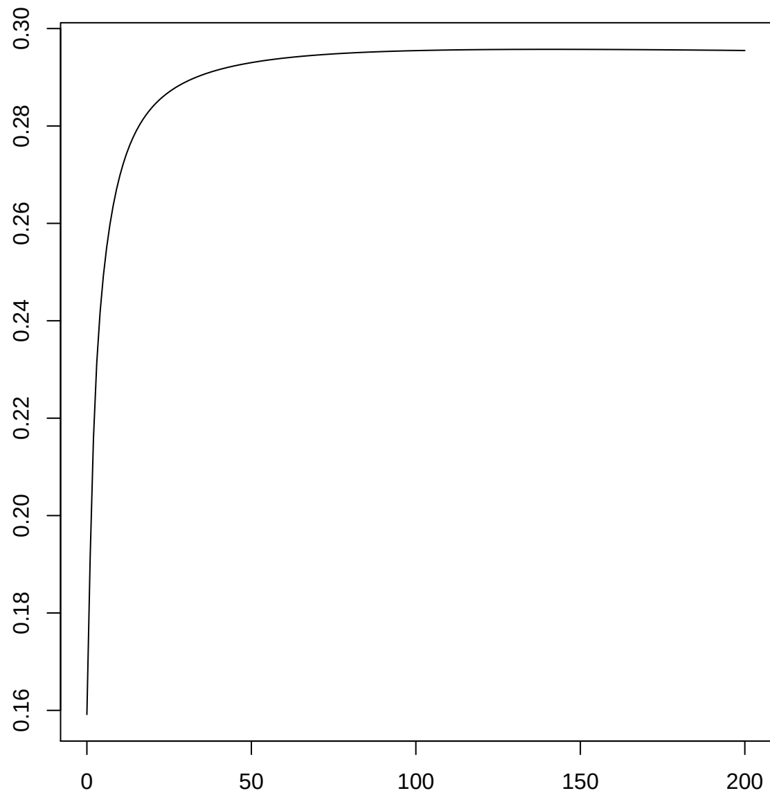
Cross validation. Squared-error loss
