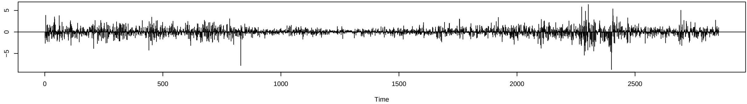
ACF of Residuals
