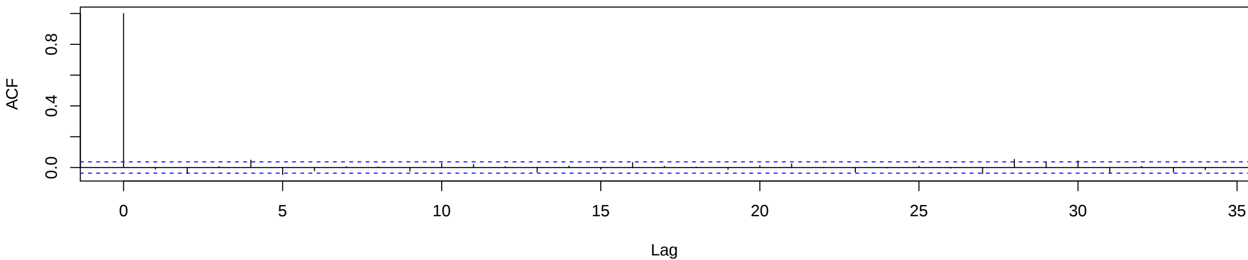
ACF of log returns of GN
