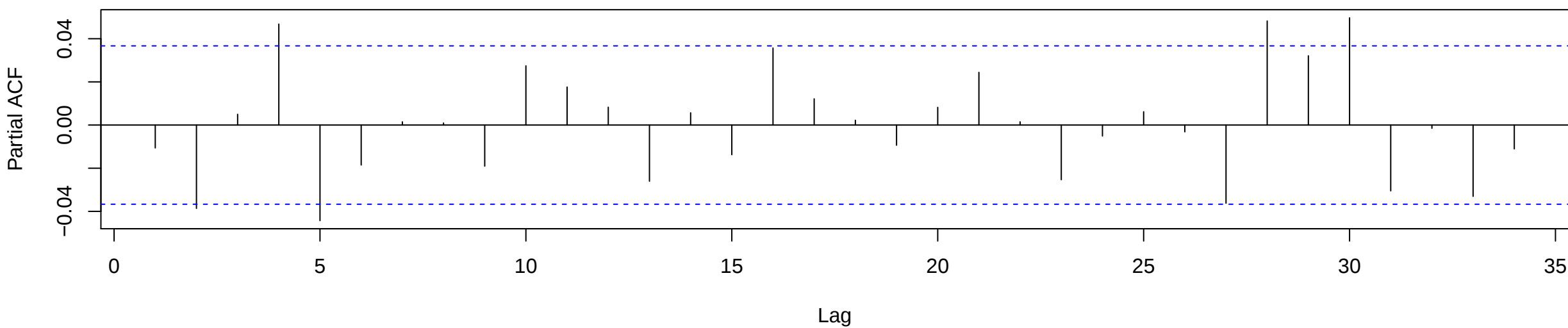
PACF of log returns of GN
