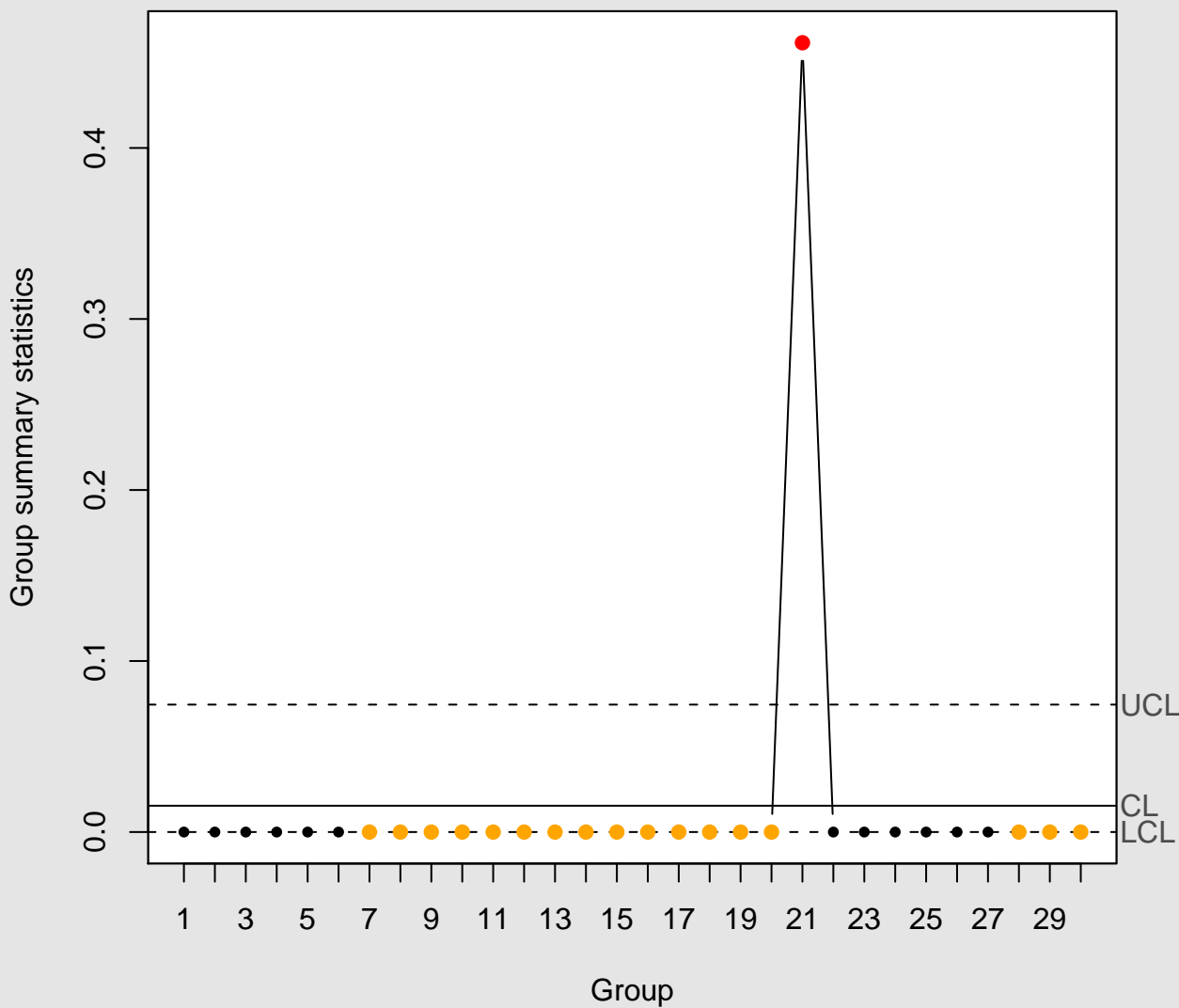
p Chart for defectuosos
