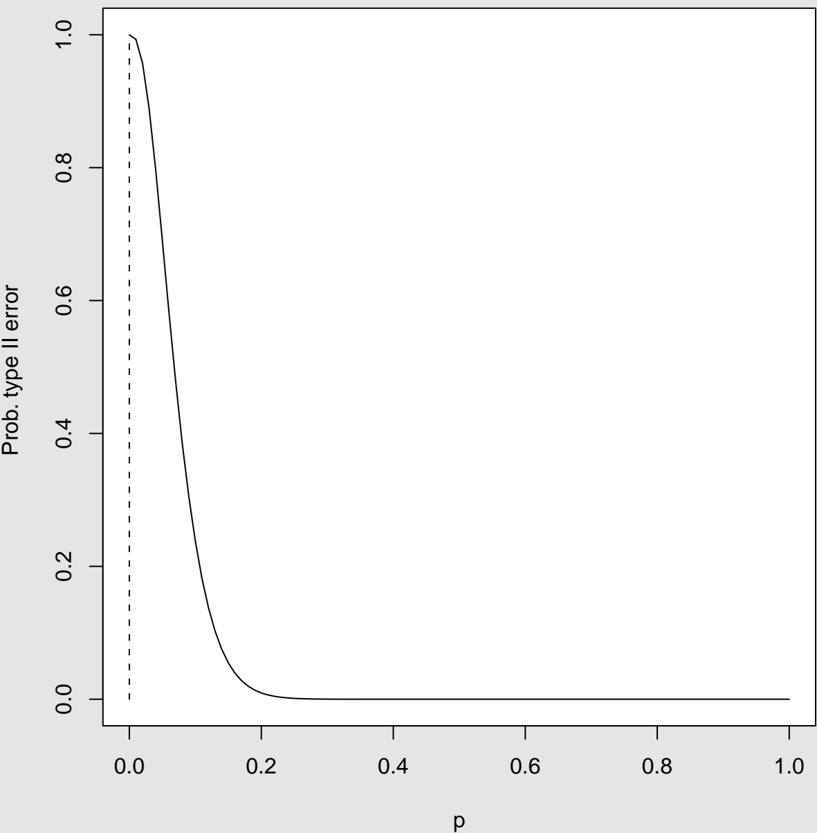
OC curves for p chart
