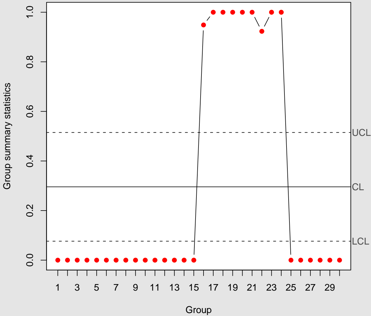
p Chart for defectuos01
