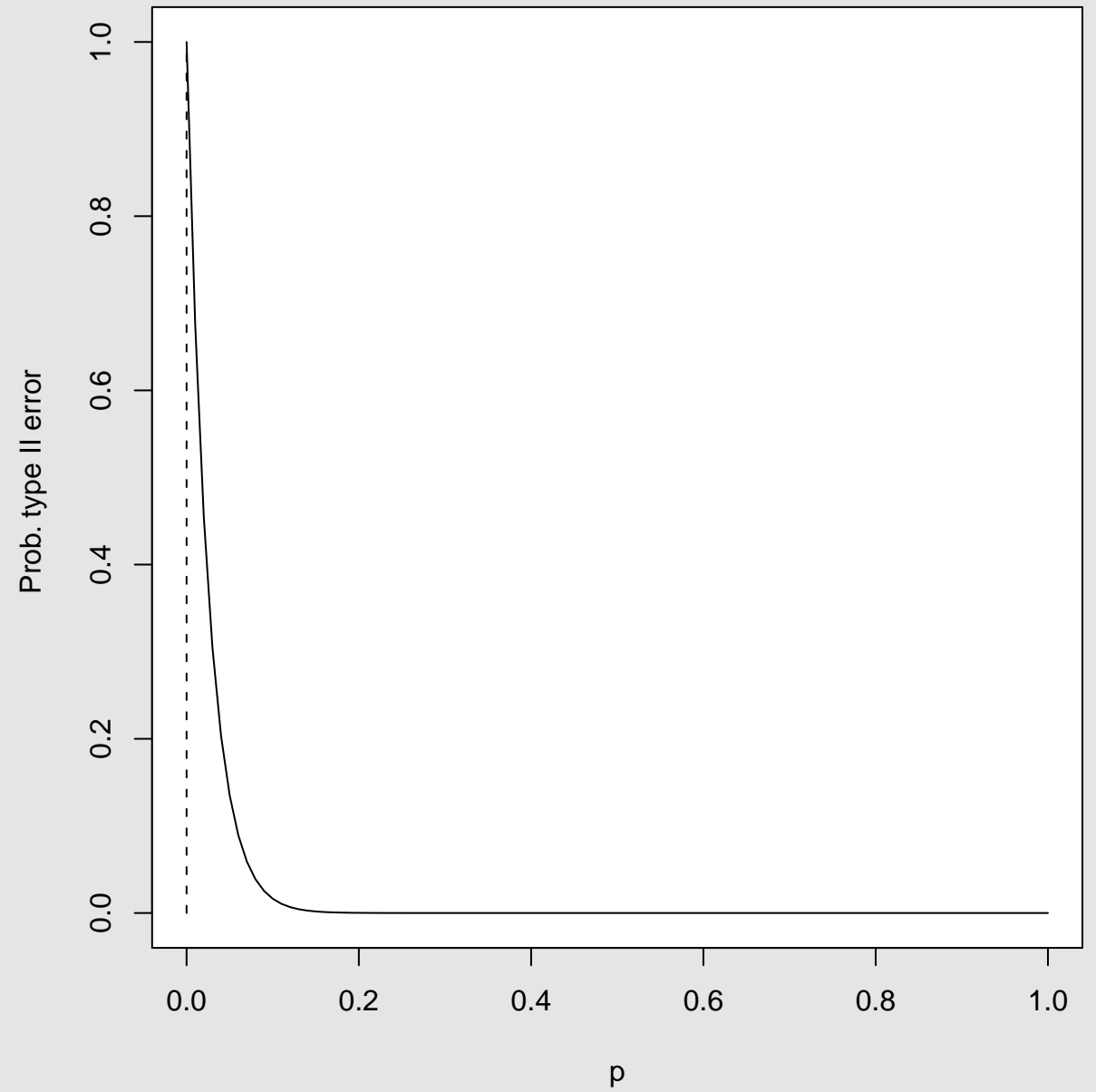
OC curves for p chart
