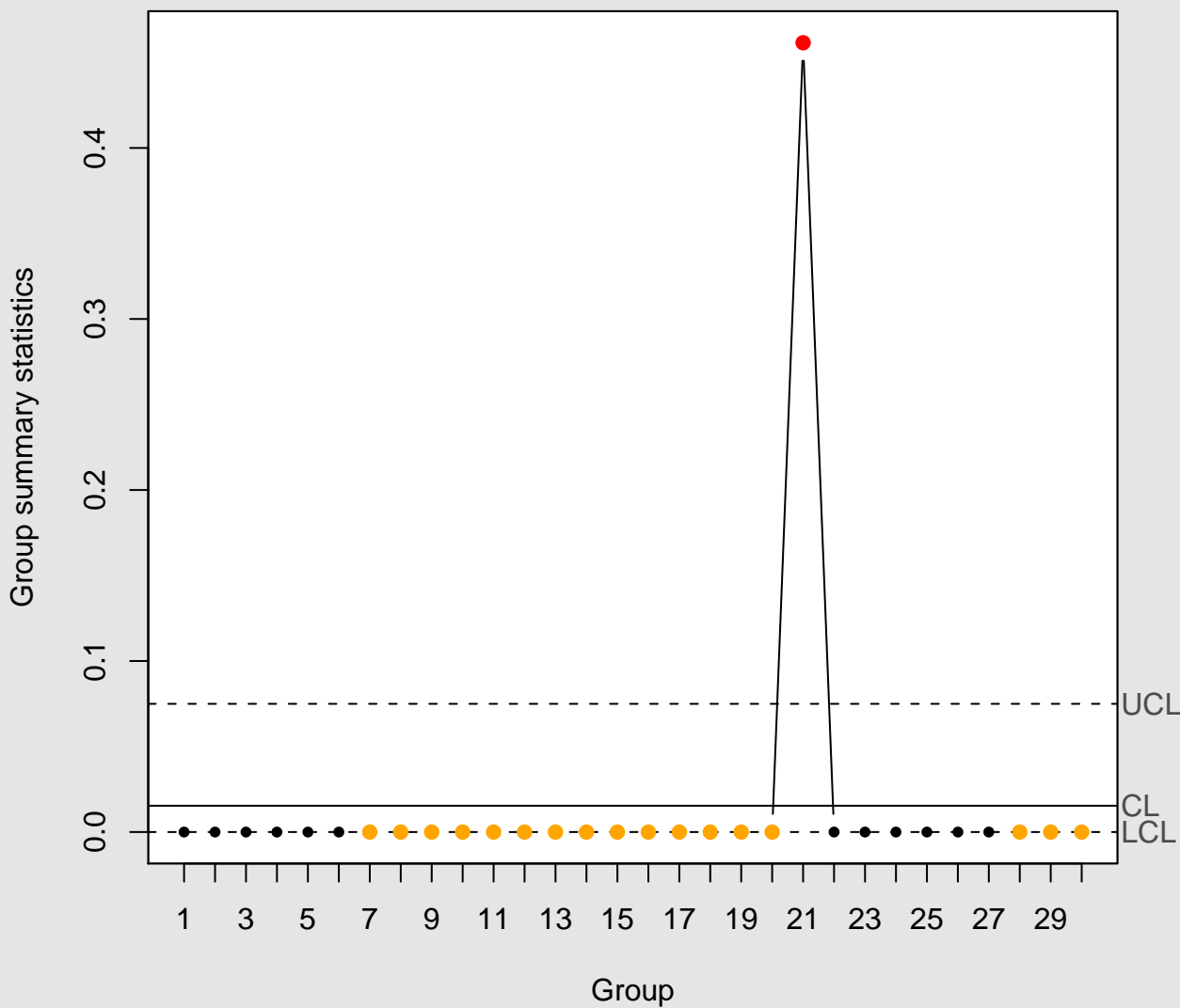
u Chart for defectuoso
