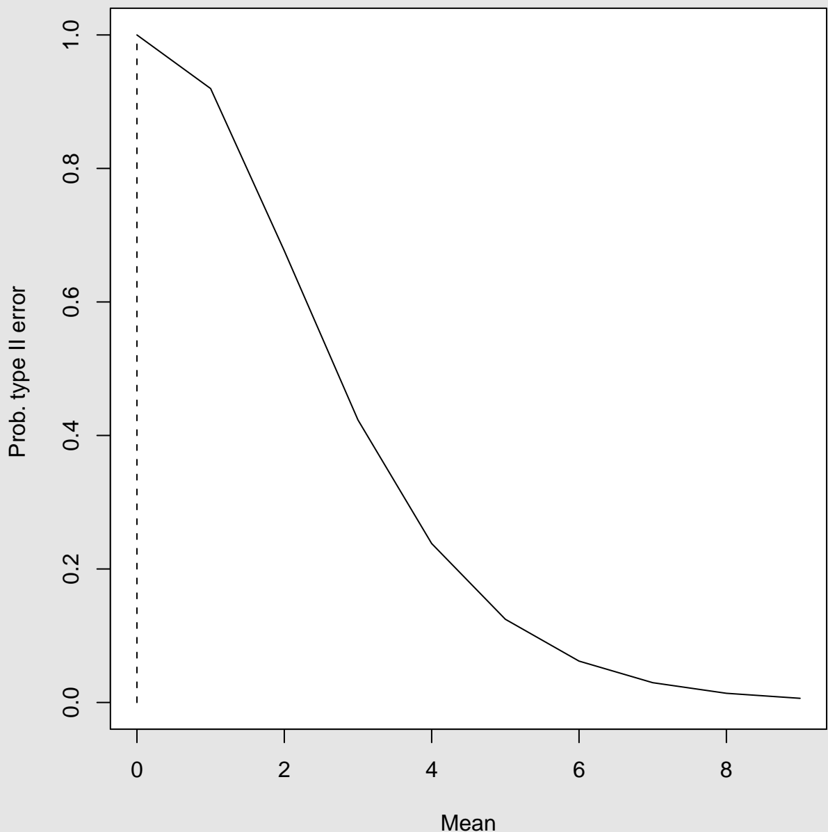
OC curves for u chart
