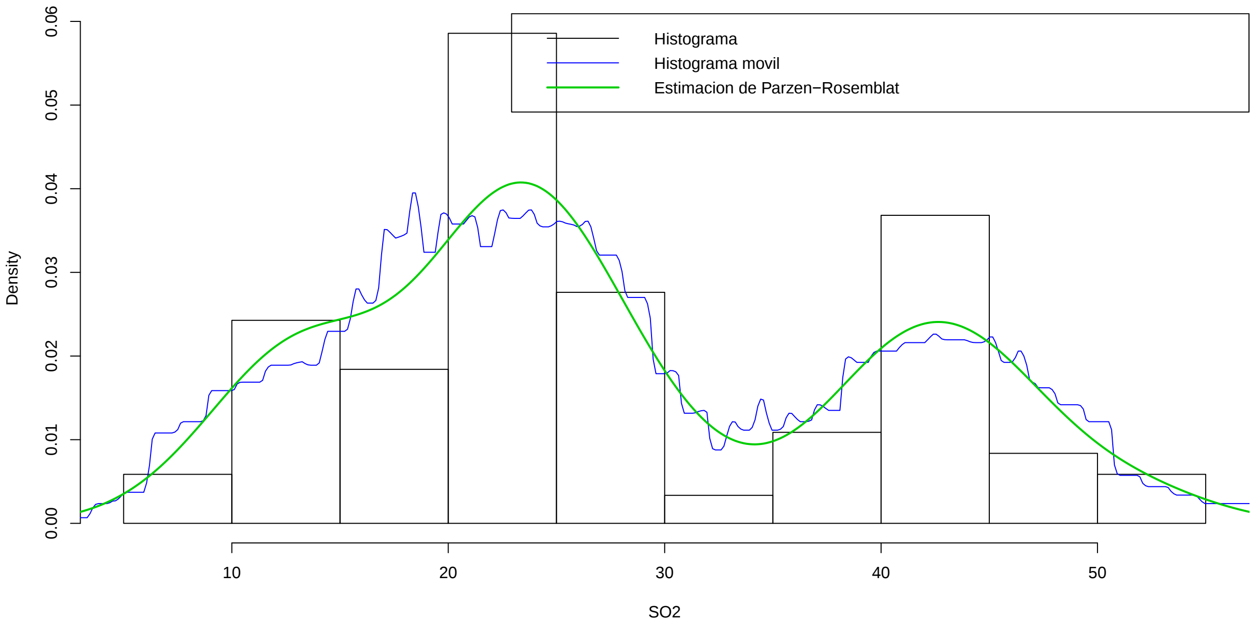
Histogram of SO2
