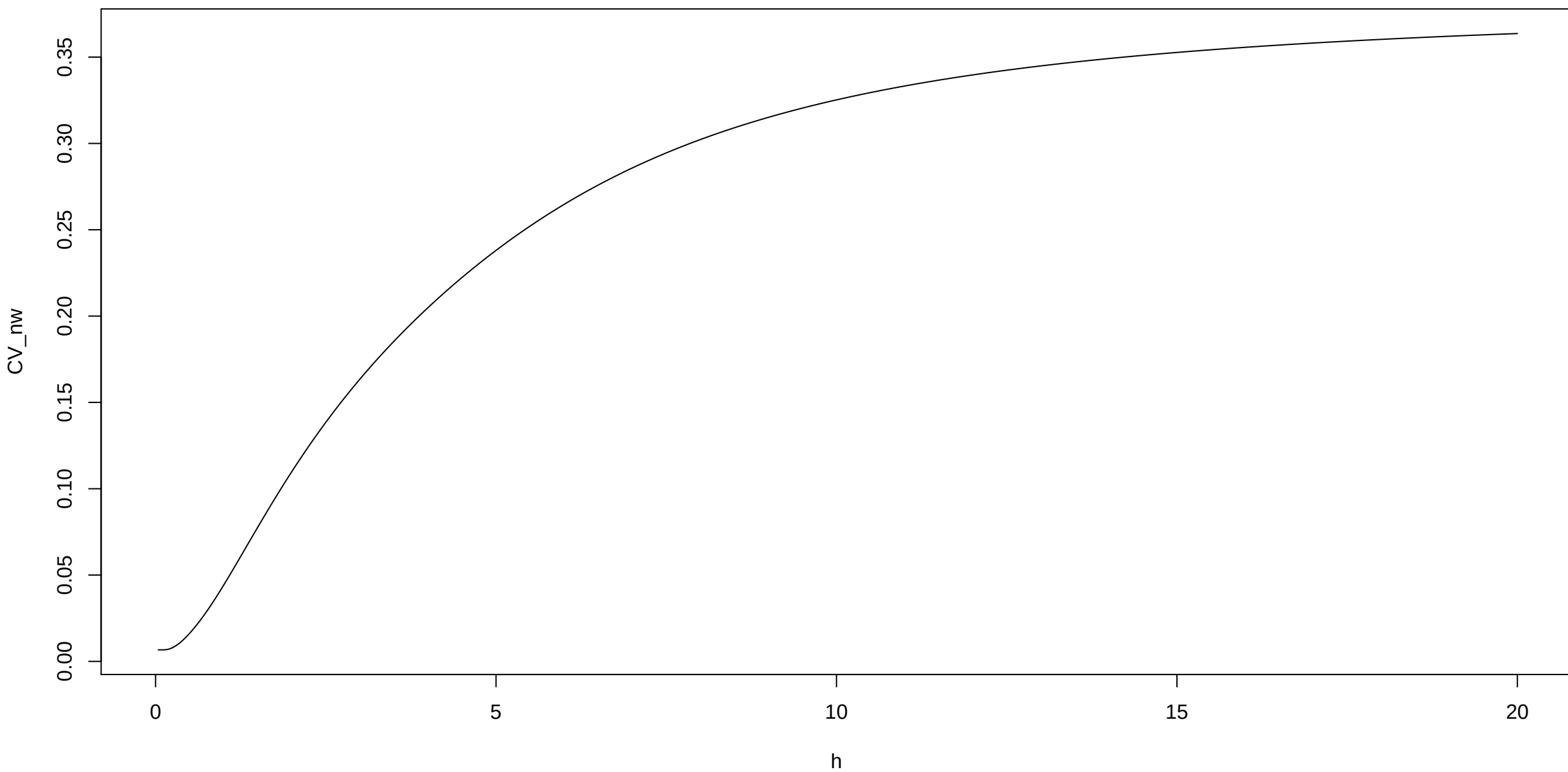
cross validation Nadaraya-Watson
