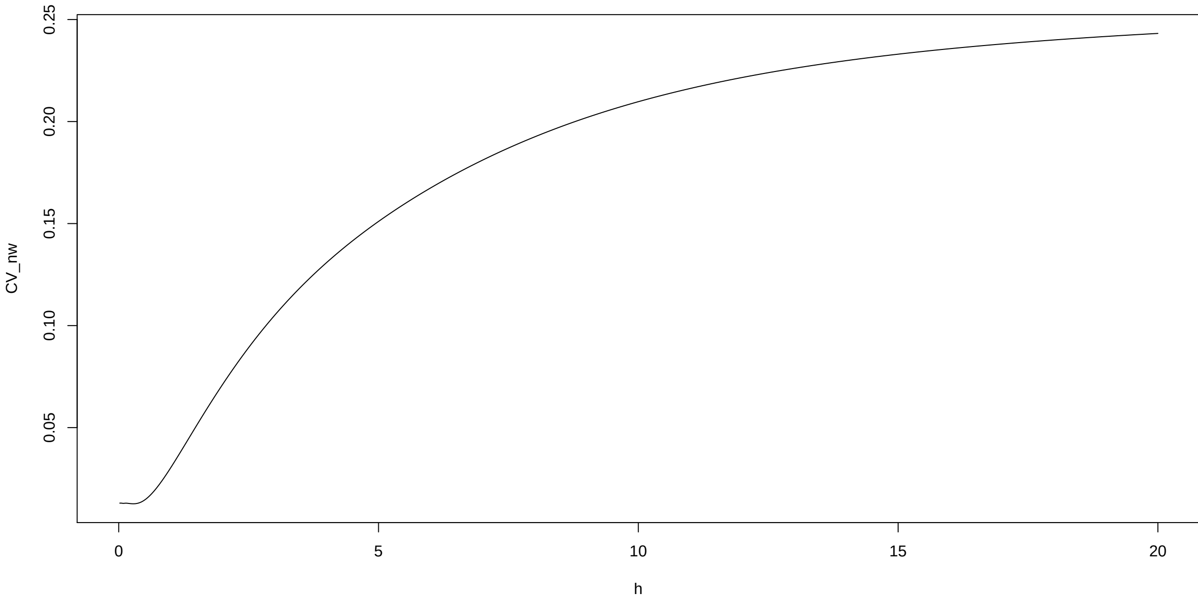
cross validation Nadaraya-Watson
