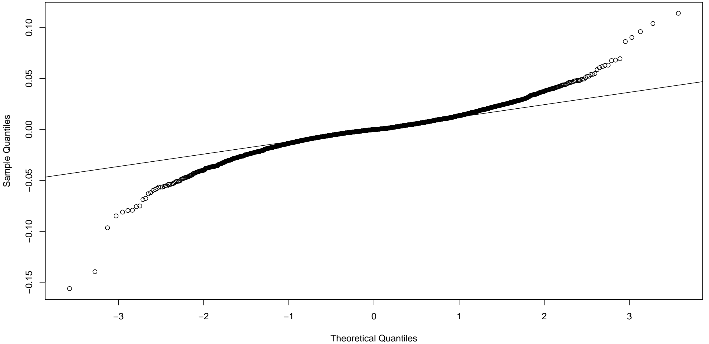
Normal Q-Q Plot
